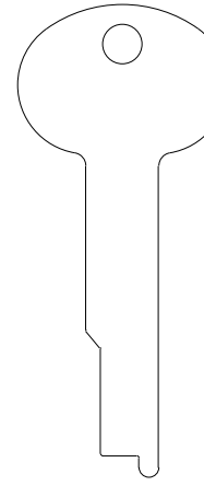
.070" - 1.8mm .280" - 7.1mm 1362
