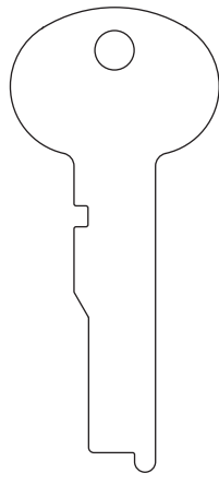
.070" - 1.8mm .320" - 8.1mm 1334
